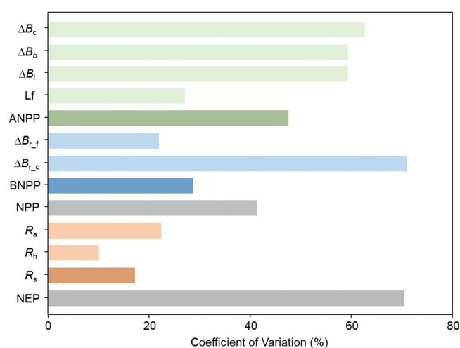
Figure 2. Coefficient of variations (CVs) in net primary production (NPP) and soil CO 2 efflux (R s ) components with net ecosystem production (NEP). See abbreviations in Materials and Methods section.
