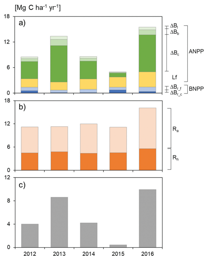
Figure 1. Year-to-year fluctuations in a) net primary production (NPP) and b) soil CO 2 efflux (R s ) components with c) net ecosystem production (NEP) for 5-years. See abbreviations in Materials and Methods section.
